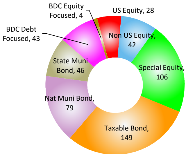
Number of Funds by Major Groupings Total CEFs 497
