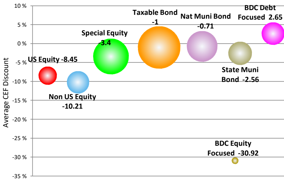
Average Discount to NAV for Major Groupings
