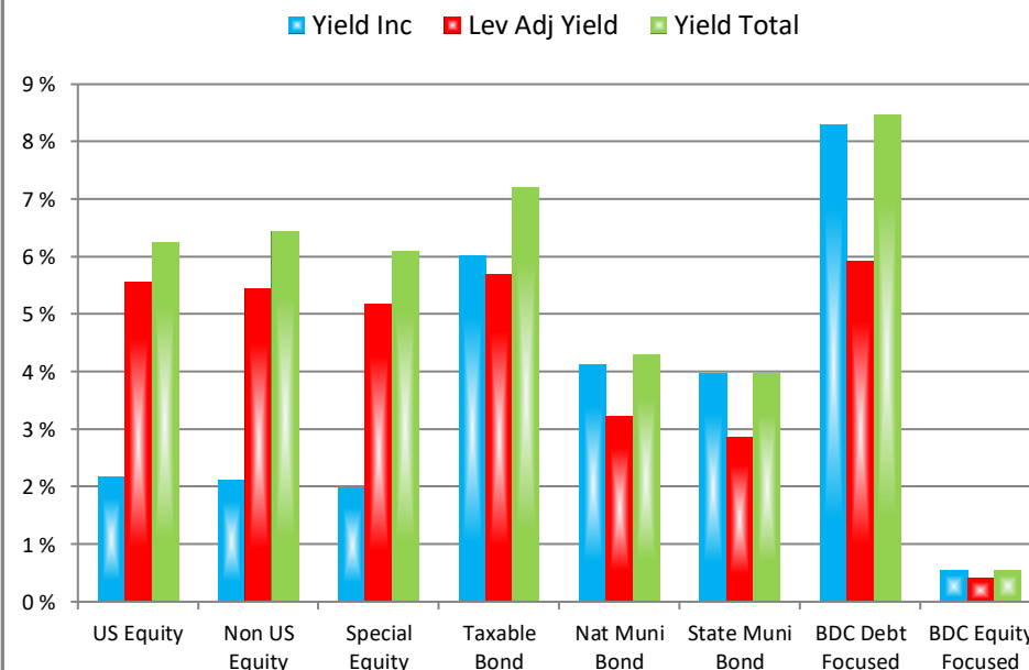
Average Yield by Major Groupings
